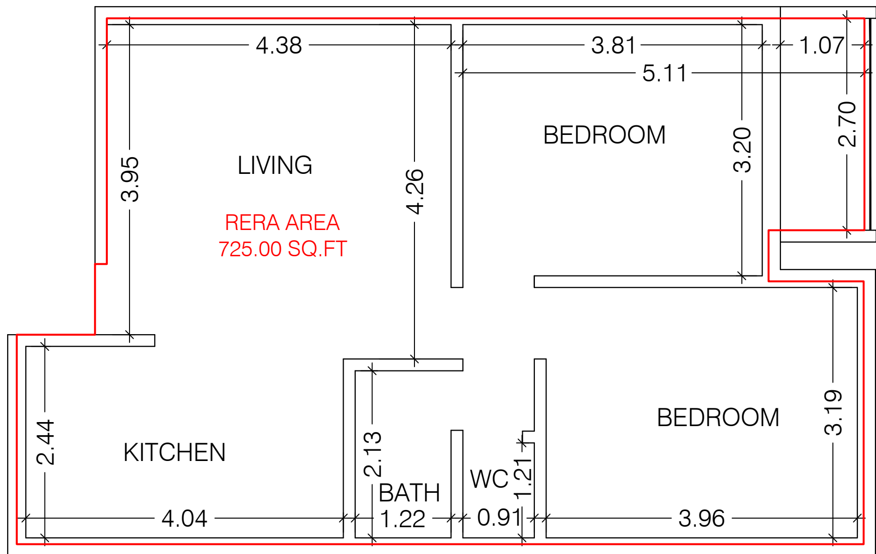
TYPICAL FIRST & SECOND FLOOR PLAN
